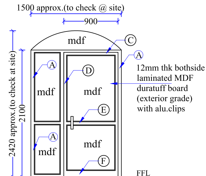
ALUMINIUM PARTITION (Size-1500x2420) WITH DOOR
