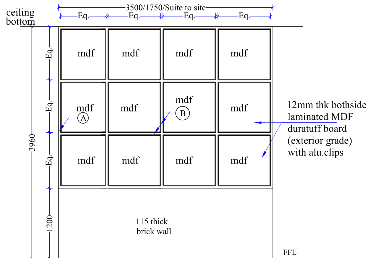
ALUMINIUM PARTITION WITHOUT DOOR- Recovery area
