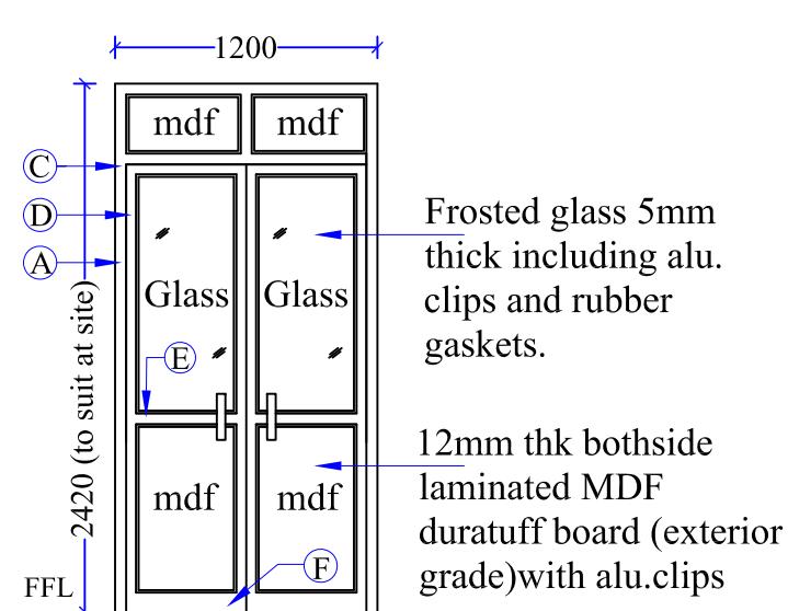
ALU. Partition 1200X2420mm with door
