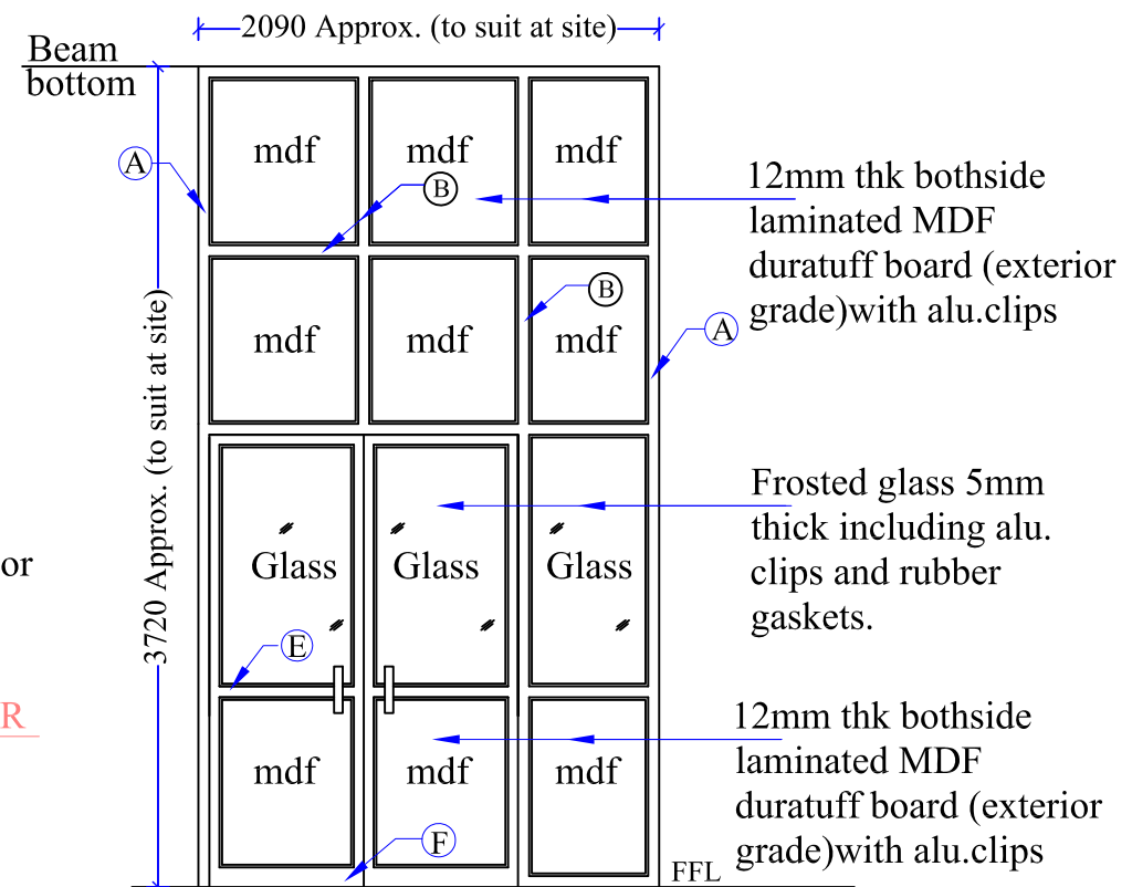
ALU. PARTITION-2 SIZE-2090X3720 WITH DOUBLE DOOR
