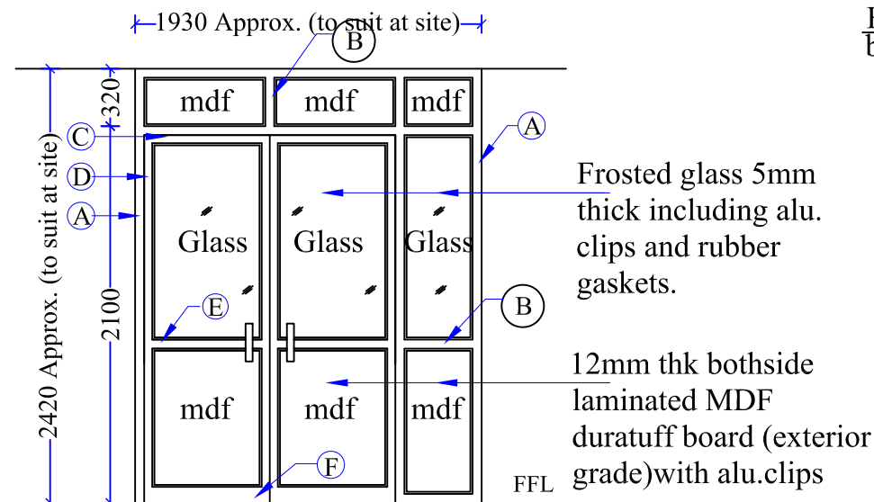
ALU. PARTITION-1 SIZE-1930X2420 WITH DOUBLE DOOR
